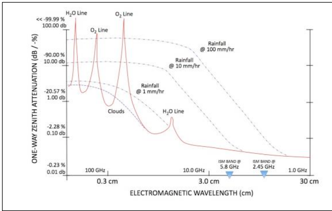
Figure 4-4 Atmospheric Attenuation of RF at Various Wavelengths
