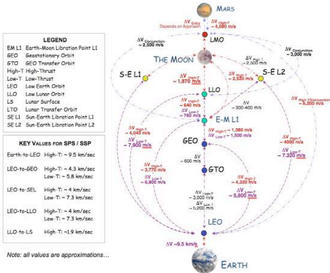
Figure 11-3 Space Transport Energy Requirements Diagram
