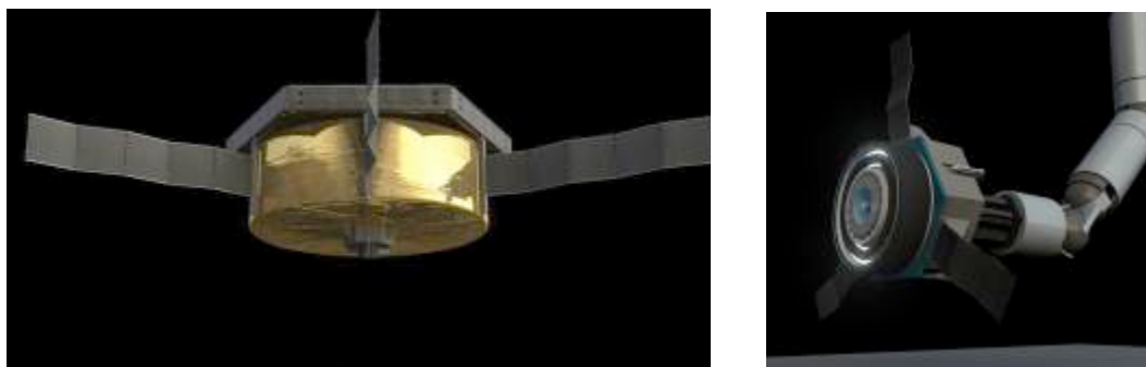
Figure 5-11 Illustrations of the “Propulsion / Attitude Control” (PAC) Concept
