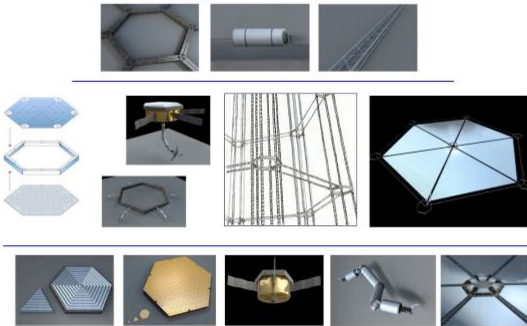
Figure 5-12 SPS-ALPHA Modules-to-Assemblies Illustration
