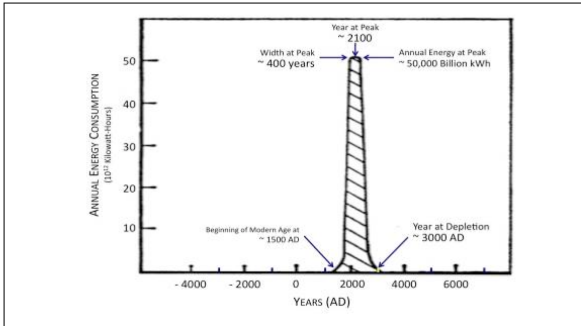
Figure 2-1 Annotated Hubbert Curve from Glaser's 1968 Science Paper
