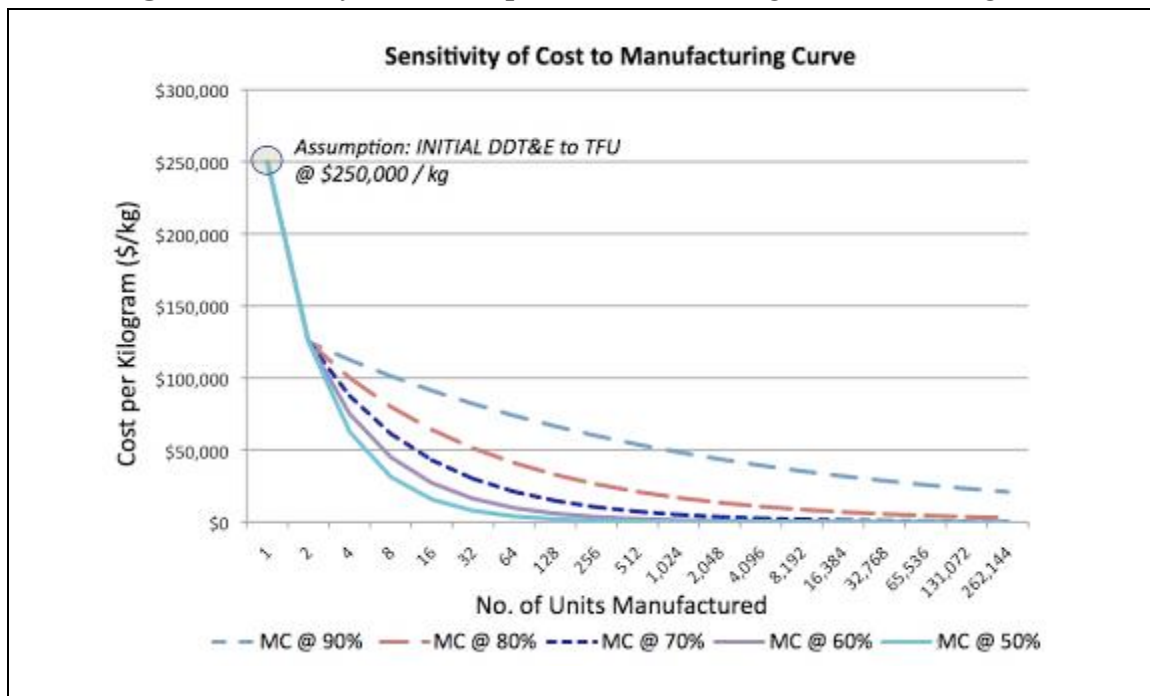
Figure 6-3 Analytical Examples of the Learning/Manufacturing Curve
