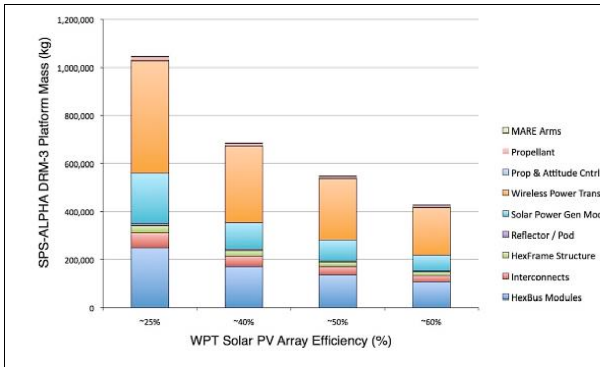
Figure 10-2 Impact of Variations in SPG Efficiency (DRM 3 @ 18 MW)
