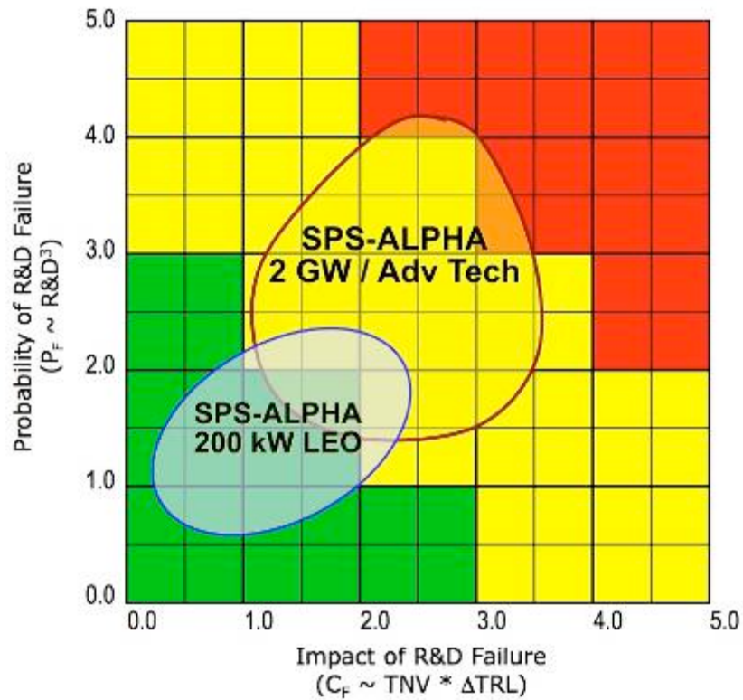
Figure 14-5 Integrated Risk Matrix for DRM-2 vs DRM-5
